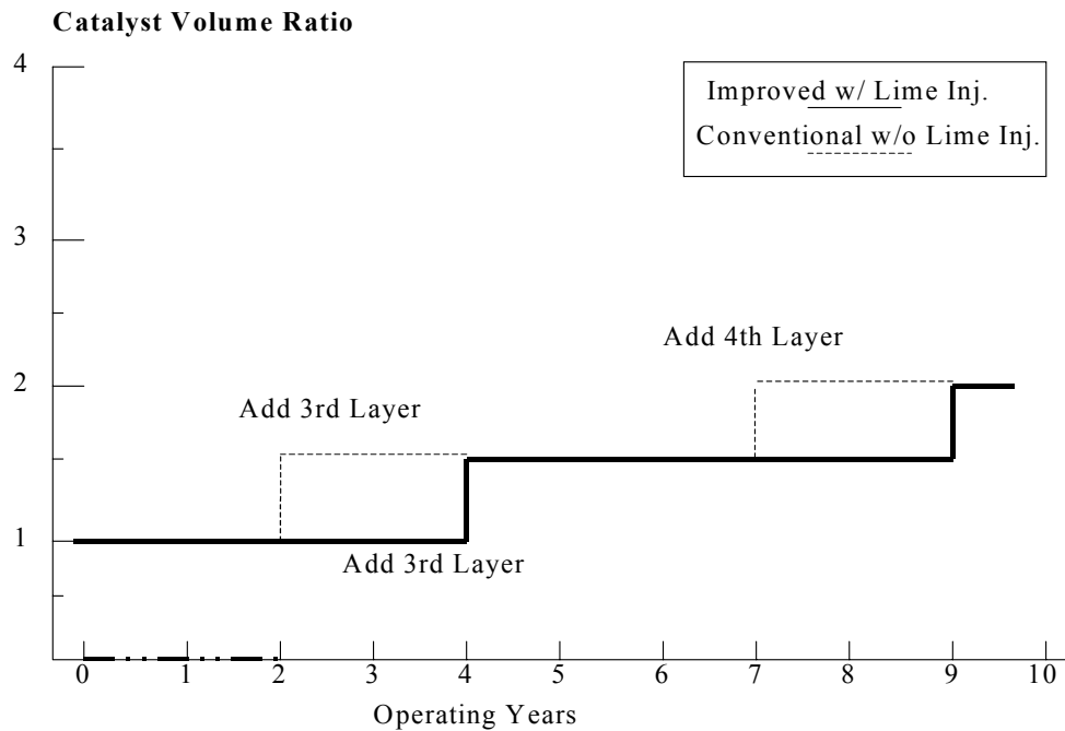
Figure 22 Impact Of Limestone Wet Bottom Boiler
