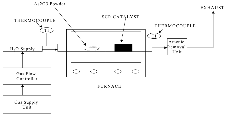
Figure 17 Schematic of Arsenic Testing Apparatus
