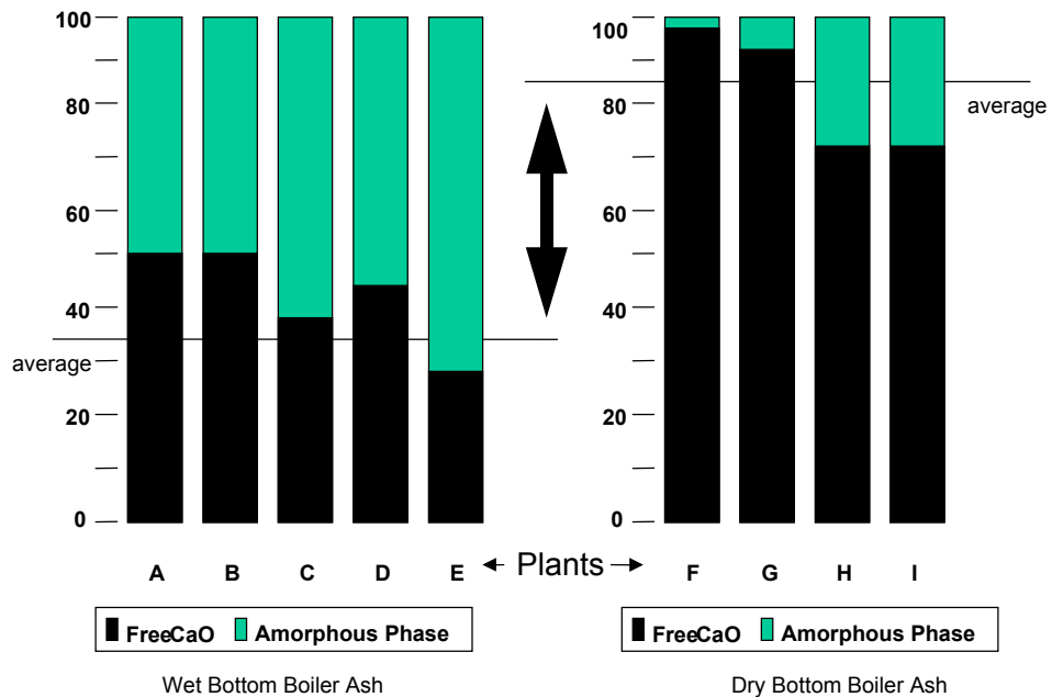
Figure 13 Free CaO Ratio in Fly Ash
