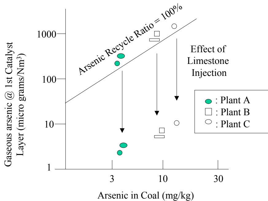
Figure 10 Relationship Between Arsenic in Coal and Gaseous Arsenic
