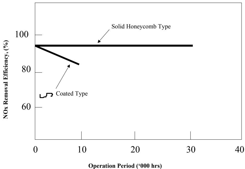
Figure 7 Comparison of Durability (Oil Firing)
