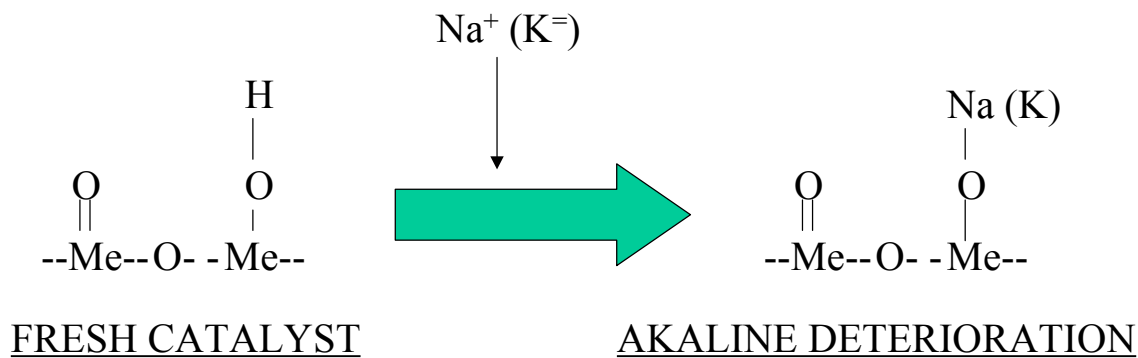
Figure 6 Alkaline Deterioration Mechanism
