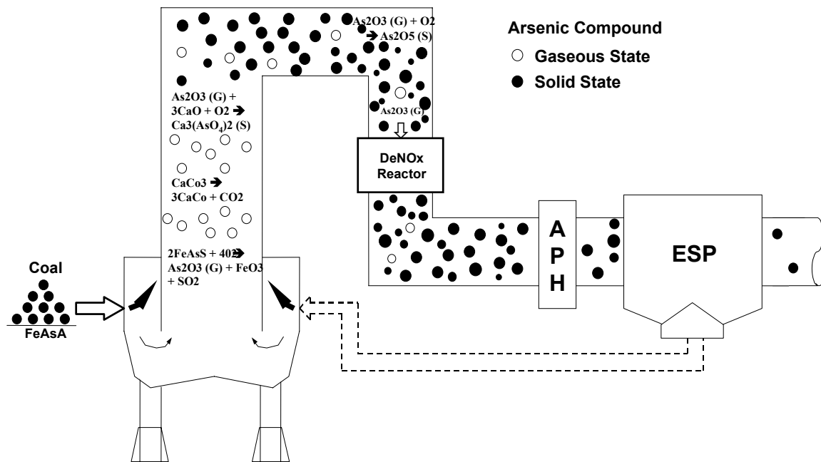
Figure 9b Effect of Limestone Injection
