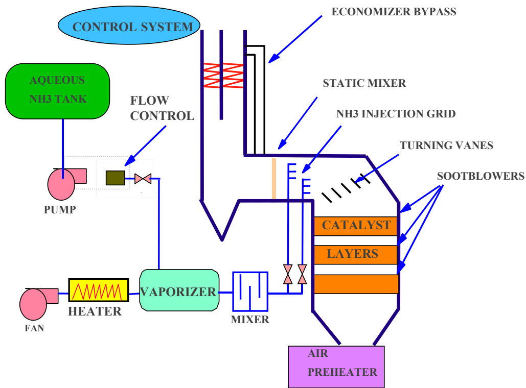
Figure 4 SCR Components
