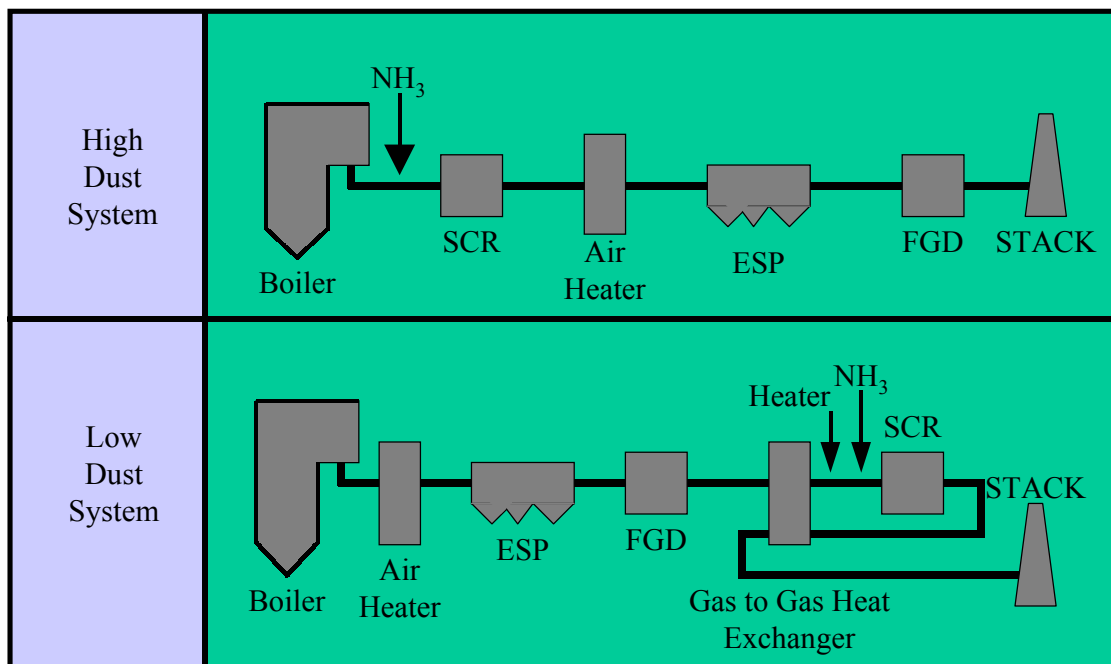
Figure 3 SCR Configurations
