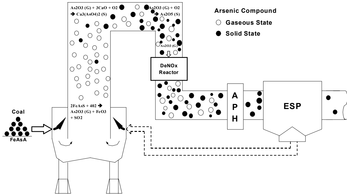
Figure 9a Arsenic Compound in Flue Gas
