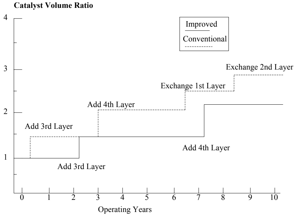
Figure 21 Impact of Improved Catalyst Wet Bottom Boiler
