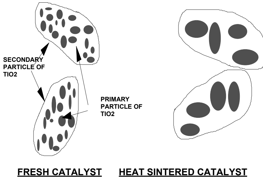
Figure 5 Thermal Sintering
