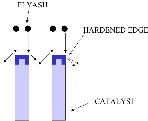
Figure 14 Honeycomb Catalyst with Hardened Edge
