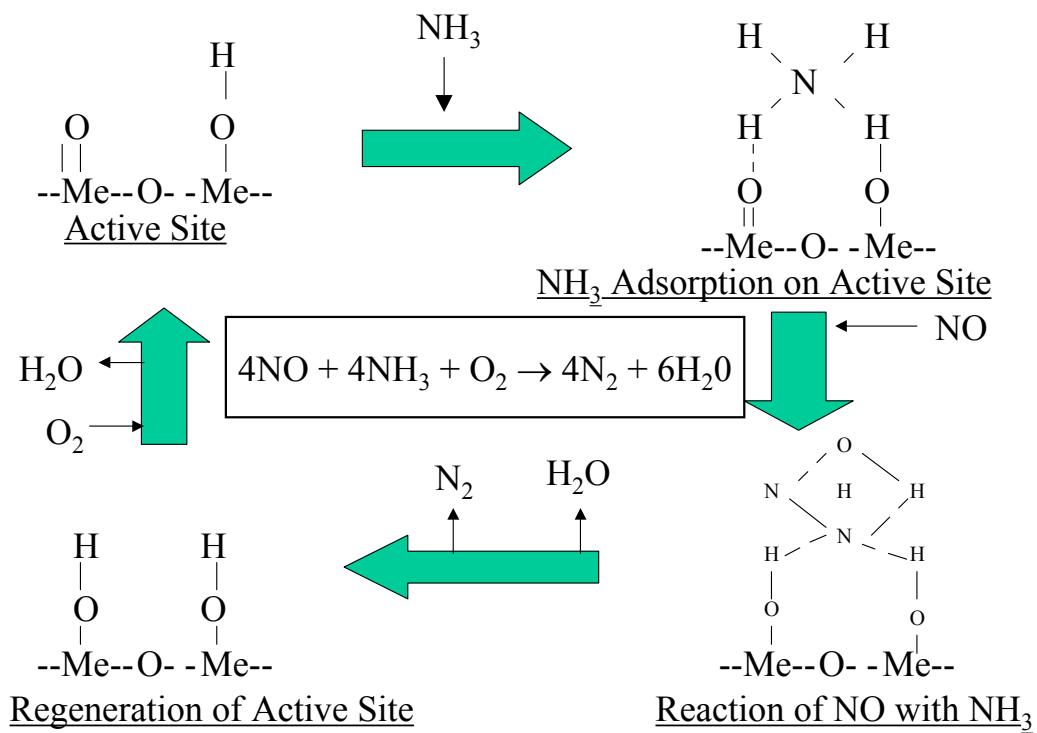
Figure 2 SCR Surface Reaction Mechanism
