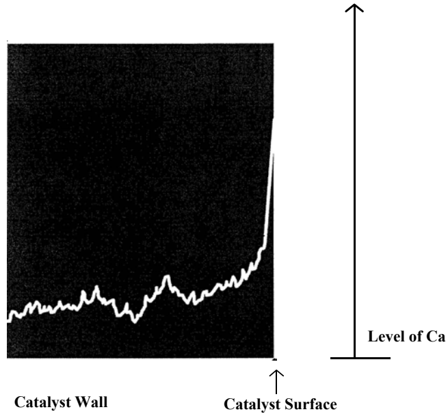
Figure 12 Accumulation of calcium Composition in Catalyst
