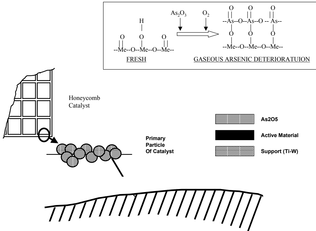
Figure 8 Model of Arsenic Compound Accumulation
